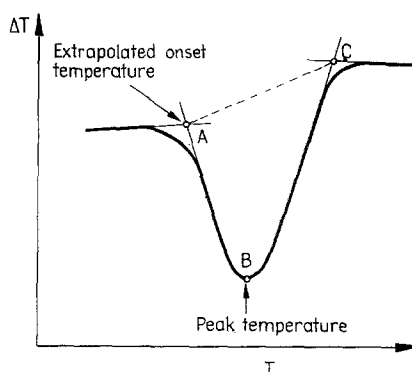
Fig. 1. Definition of temperatures and peak area used in ICTA International Test Program
